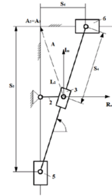
Fig 9.:Mechanism that corresponds to the problem from Fig 8.
