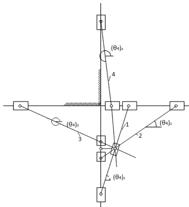
Fig. 14. :Solution of the mechanism positions
