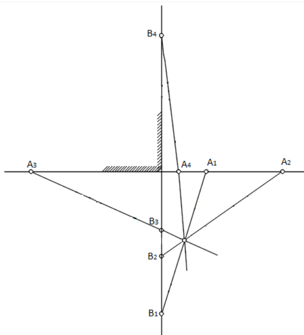
Fig. 15. :Solution of the starting geometric problem
