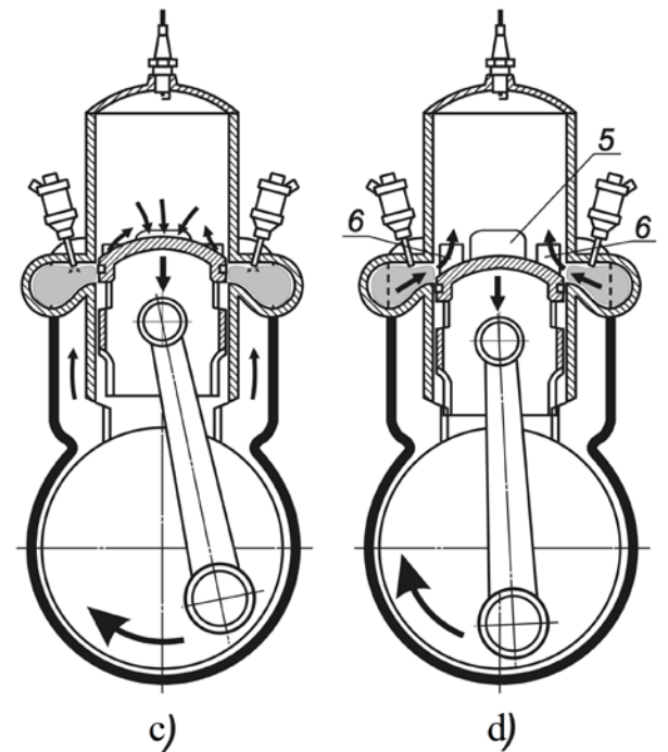
Fig. 3. The scheme of work of the engine with the stratification of the fresh charge and the cumulative chambers: 1 – cumulative chambers; 2 – electromagnetic nozzles; 3 – the inlet port clean air; 4 – ports in piston; 5 – the outlet port; 6 – vent windows
