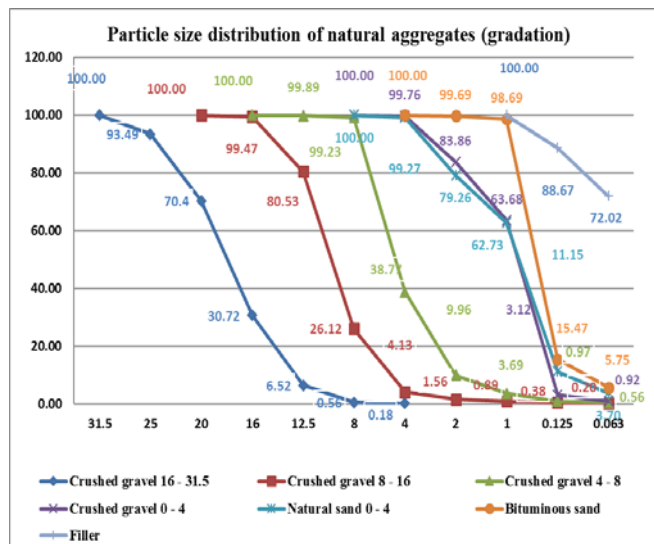
Fig. 3 – Particle size distribution of natural aggregates (gradation)
