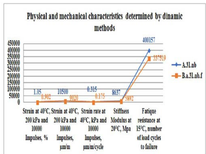
Fig. 6 – Values of physical and mechanical characteristics determined by dynamic methods
