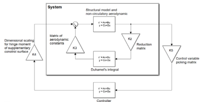
Fig. 2 Schema of the closed-loop model
