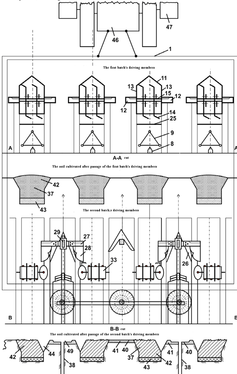
Fig. 3. Mounting Arrangement of Driving Members of Batch-Combined Machine:
