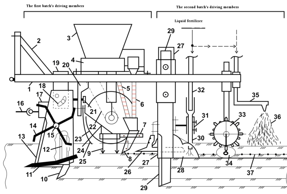
Fig. 2. The Scheme of Batch-Combined Machine for Strip Tilling-Sowing and Crop Tending:
