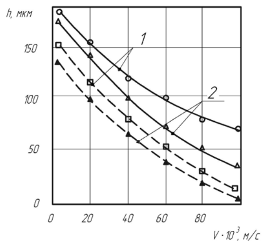
Fig.6. The dependence of the thickness of the melted layer in the elements of the optical glasses BK10 (1) and TF110 (2) on the speed of the electron beam: ——— F_n = 6 \cdot 10^8 Wt/m 2 ; - - - - F_n = 3 \cdot 10^8 Wt/m 2 ; Δ, ○, □ – experimental points.
