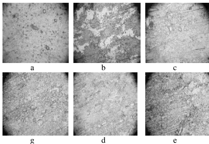
Fig. 2 The morphology of the surface layer of a sample of steel 45 with an under layer of TiN without dropping phase, modified oligomer F-14, after frictional engagement with a graphite sample: a - the original; b - after 10 cycles; c - after 20 cycles; g - after 30 cycles; d - after 40 cycles; e - after 50 cycles. \times 300
