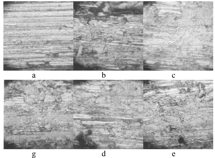
Fig. 4 The morphology of the surface layer of a sample of steel 45 with a sub layer of TiN without dropping phase, modified by oligomer F-1, after the frictional interaction with composites based on PTFE: a - the original; b - after 10 cycles; c - after 20 cycles; g - after 30 cycles; d - after 40 cycles; e - after 50 cycles. \times 300
