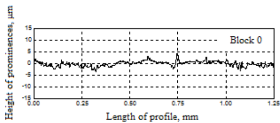
Fig. 11 Representation of topography of the block 0 in the new condition.
