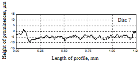
Fig. 10 Representation of topography of the disc 7 in the worn condition.
