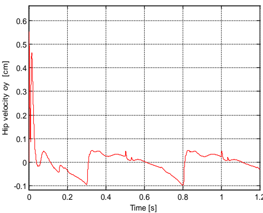
Fig.6 Hip velocity in direction y
