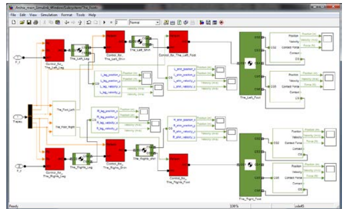
Fig.7 The Subsystem for feet with ground
