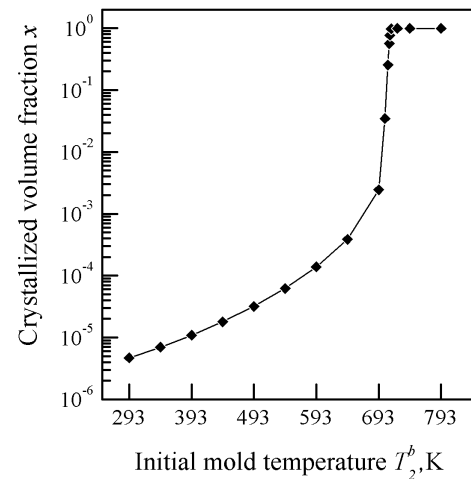
Figure 2 – Dependence of the crystallized volume fraction vs. the initial temperature of the ingot mold for castings with a half-thickness of 550 \mu\text{m} .
