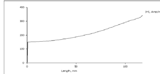
Fig. 20. Magnetic flux distribution in transformer at first leg- rated load.
