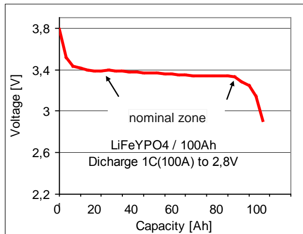
Figure 1. Typical dilution curve of lithium-ion battery LiFeYPO4
