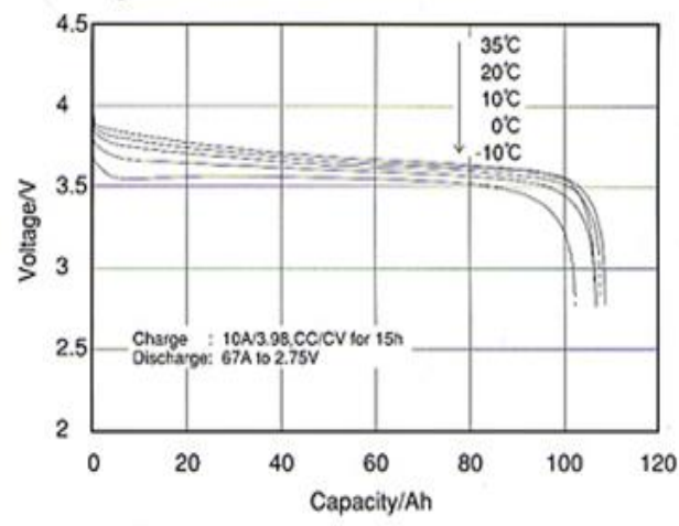
Discharge characteristics of 100Ah Li-ion cell.
