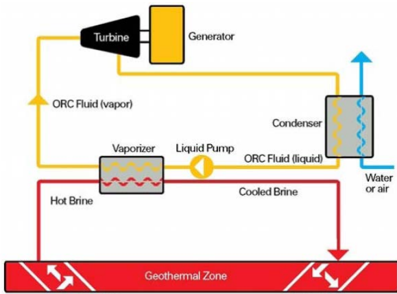
Fig. 4 ORC power station without heat regeneration [10].
