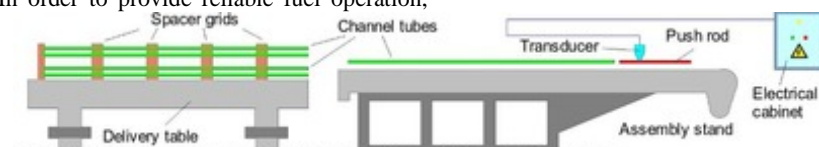
Fig. 5. Ultrasonic equipment for friction reduction for fuel assemblies manufacturing
