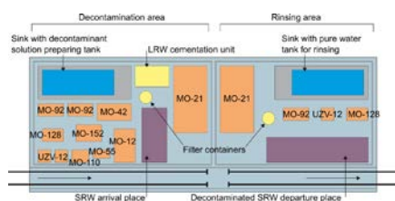
Fig. 17. Draft of a possible decontamination unit for metal parts
