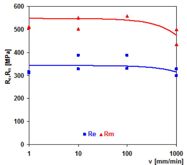
Fig. 6 Dependence of mechanical properties on the loading rate in the modified bending test.
