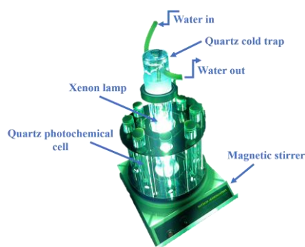
Fig. 1. TOPT-V photoreactor
