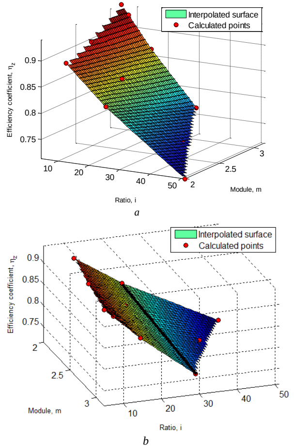
Fig. 3. Efficiency coefficient in relation from ratio and module for center distance a = 63 mm and rotation speed n_1 = 1500 \text{ min}^{-1} .
