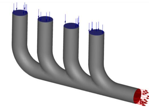
Fig. 7 Inlets and outlet for Exhaust manifold A
