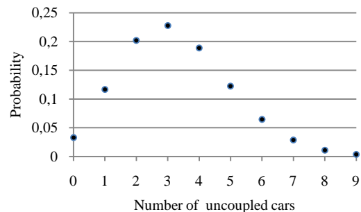
Fig.2 Probability of uncoupling of various numbers of cars from a car batch.
